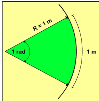
Gambar 2.44 Radian
