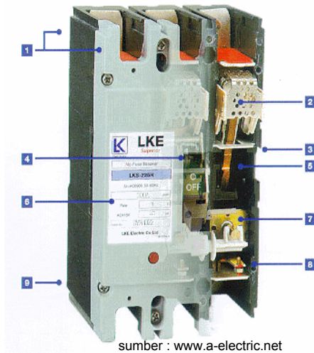
Gambar 2.22 Moulded Case Circuit Breaker
