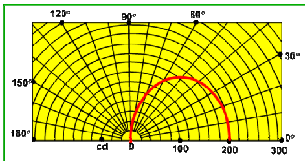
Gambar 2.53 Diagram Polar Intensitas Cahaya Lampu Pijar
